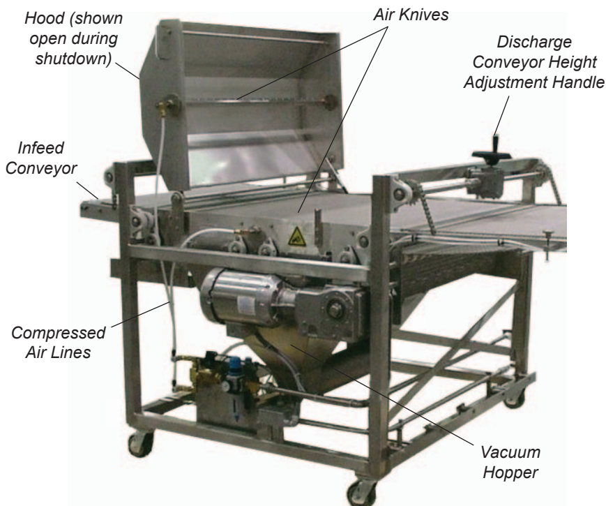
Flour Removal Conveyor (using compressed air)
